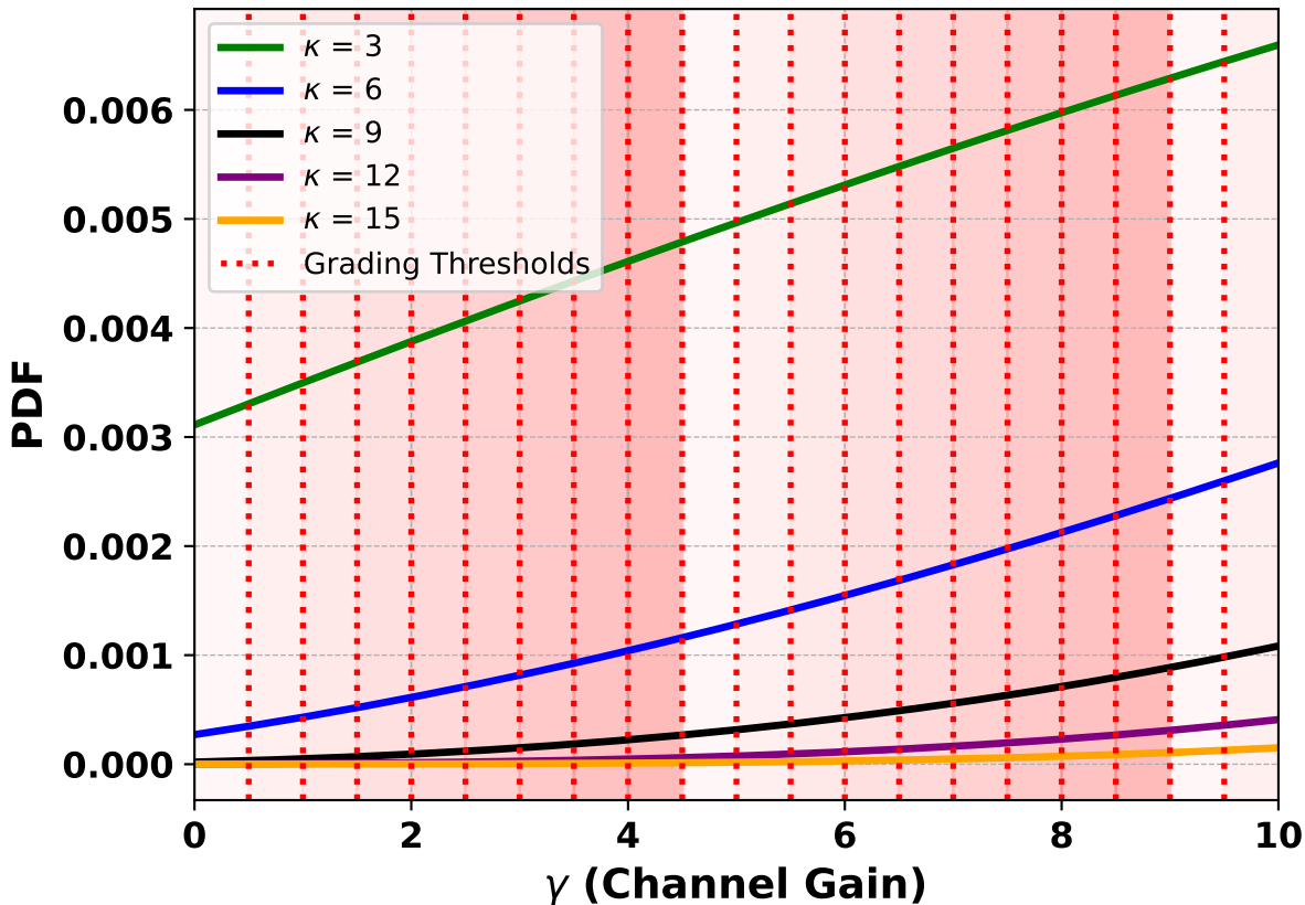
PDF of \gamma with d = 8.0
